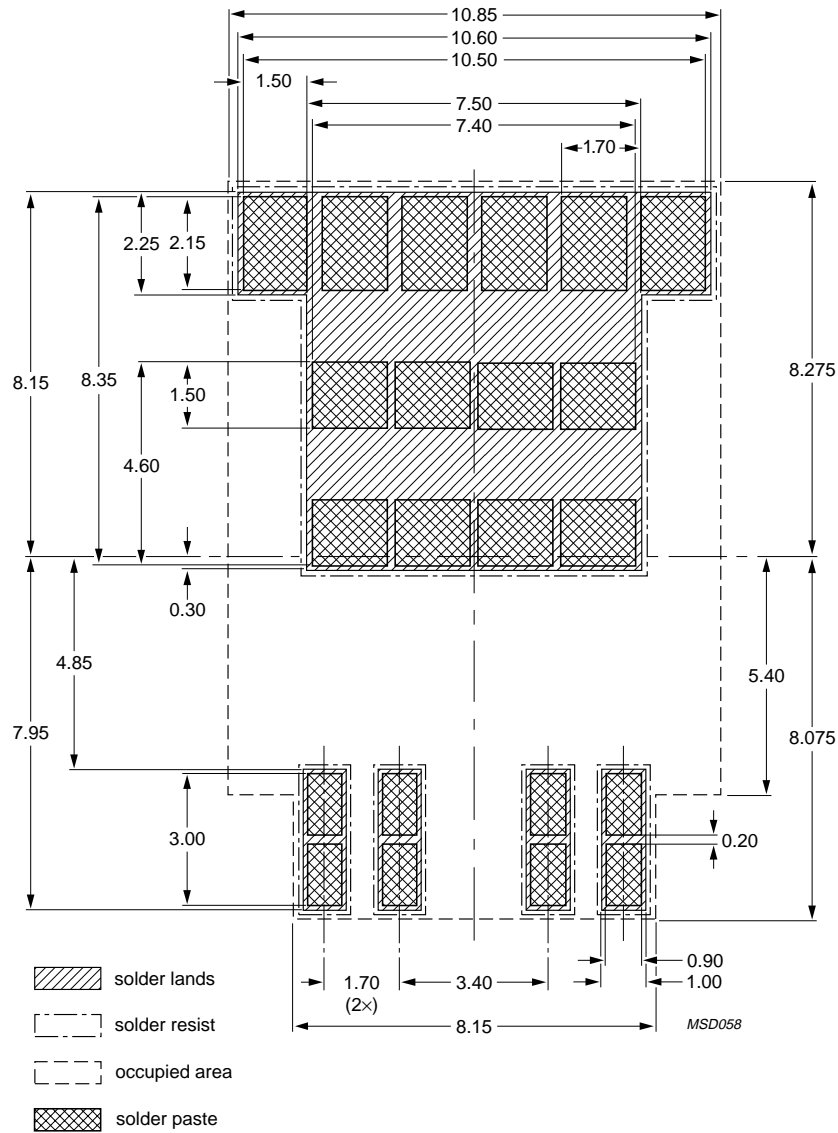
Fig 20. Reflow soldering footprint for SOT426.
